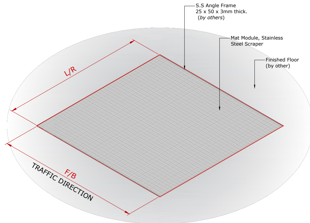
ISOMETRIC DIAGRAM
