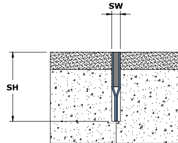
Straight Application XEA (Aluminum)
