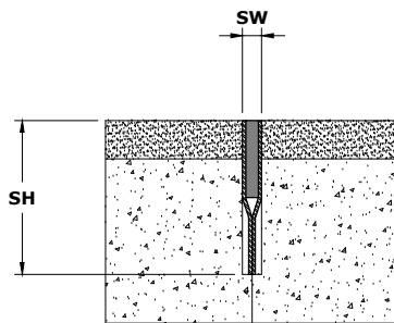
Straight Application XES (Stainless Steel)
