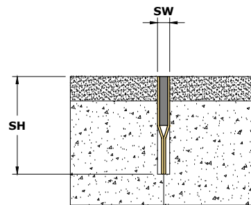
Straight Application XEB (Brass)
