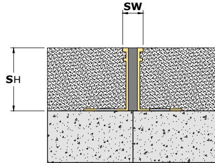
Straight Application XYB (Brass)
