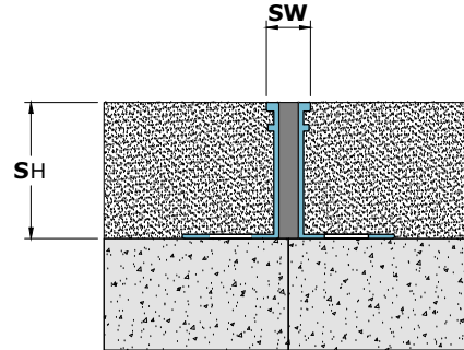
Straight Application XYA (Aluminum)
