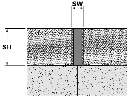
Straight Application XYS (Stainless)
