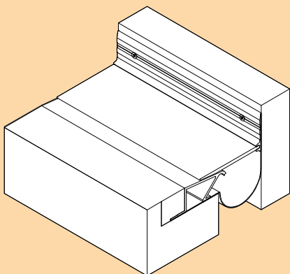
Fig. 5 - (Completed Installation)
