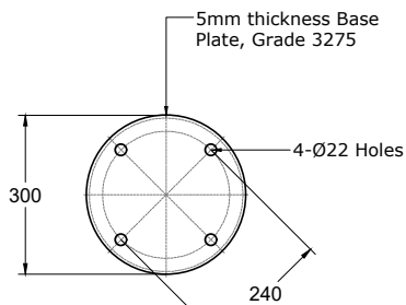
Base Plate
