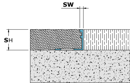
Straight Application XAA (Aluminum)
