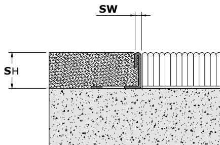
Straight Application XAS (Stainless)
