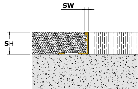
Straight Application XAB (Brass)
