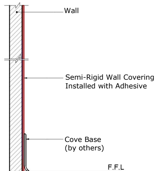
SECTION DETAIL
