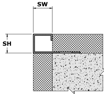
Corner Application XBS (Stainless Steel)
