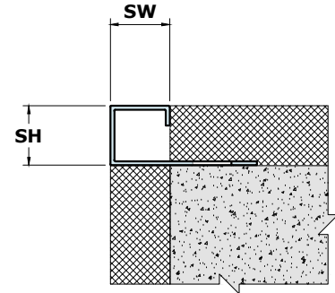
Corner Application XBA (Aluminum)
