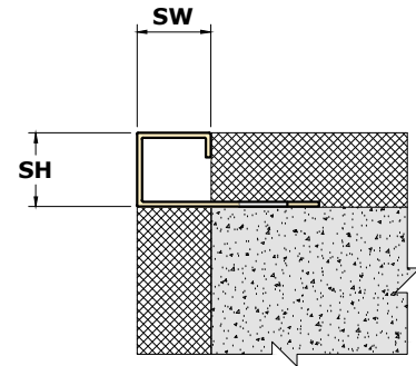
Corner Application XBB (Brass)
