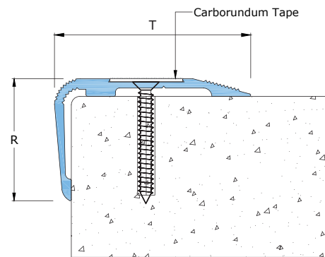
Screwdown Fixing
